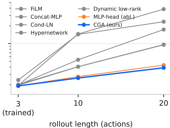
With consistency loss
