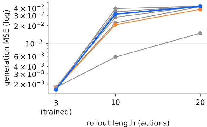
Without consistency loss
