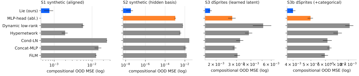
Figure 1: Compositional OOD error by conditioner across suites (log scale; bars: mean \pm sd over 10 seeds; blue = ours, orange = mechanism ablation). Lie conditioning is lowest in every suite — by five orders of magnitude when conditions form a group (S2), and by a robust margin on real-image suites with learned latents.
