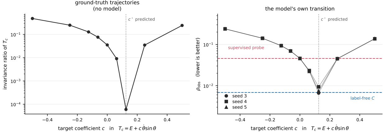
Figure 2: The model’s transition conserves the integrator’s shadow Hamiltonian, not textbook energy. Both panels sweep the target T_c = E + c \dot{\theta} \sin \theta ; the dotted line is c^* = 0.125 predicted from the integrator with no fitting. Left: on ground-truth trajectories, with no model involved, T_{c^*} is 591\times better conserved than textbook energy. Right: the learned transition agrees, on all three seeds. The sweep passes from the supervised probe’s level (red) down to the label-free scalar’s (blue) exactly at c^* . The wrong-sign control at c = -c^* is 12\times worse (median over seeds), so this is not monotone in |c| .
