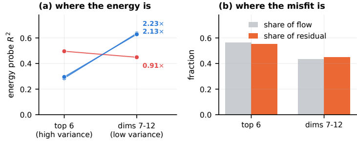
Figure 4: (a) Energy-probe R^2 for the top six principal directions against directions 7–12, per model. (b) Fraction of latent flow and pairing residual carried by each group, medians over three models.
