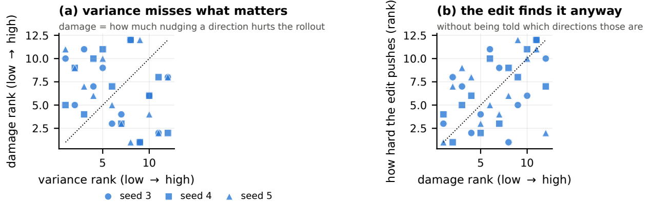
Figure 3: Each point is one of the 12 extracted directions, ranked within its own model; the dotted line marks equal ranks. (a) Variance rank against damage rank at a 40-step horizon. (b) Damage rank against the magnitude of the invariant correction along that direction.
