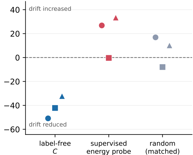
effect on imagined physics % change in energy drift
