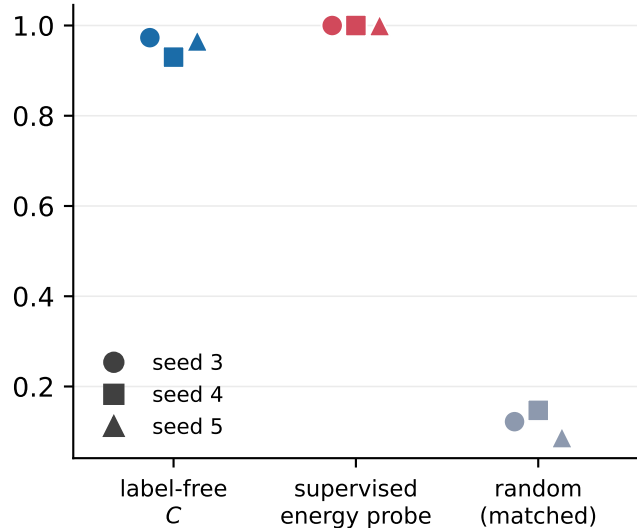
probe quality |\rho| with true energy
