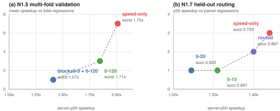
Figure 4: Speed-risk Pareto view of tactic selection. Left: N1.5 multi-fold validation shows that speed-only execution is fastest but has the largest paired regression count, while protected tactics trade speed for behavior. Right: N1.7 held-out validation shows the same structure and adds a task-conditioned tactic router as a high-speed trade-off point.
