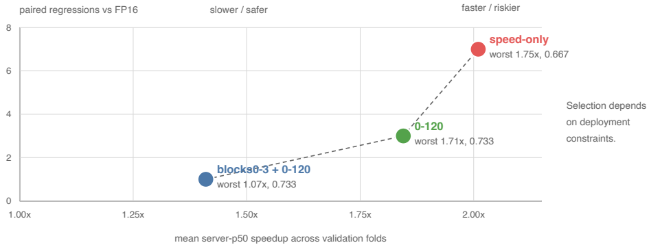
Figure 4: Speed-risk Pareto view of the multi-fold tactic search. Speed-only execution is fastest but has the largest paired regression count. The combined tactic is behavior-conservative but gives up speed. The 0–120 duration tactic is the speed-constrained compromise.
