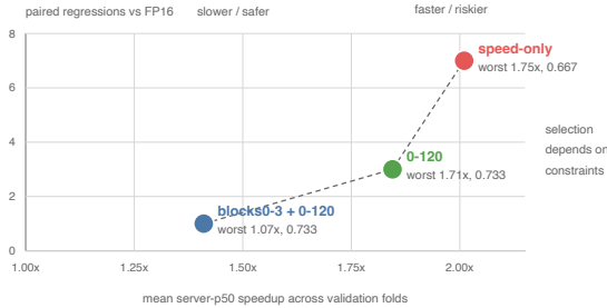
Figure 3: Speed-risk Pareto view of held-out tactic selection. Speed-only is fastest but has the largest paired regression count. The combined tactic is behavior-conservative but gives up speed. The 0–120 duration tactic is the speed-constrained compromise.
