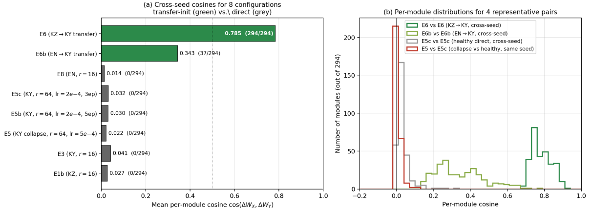
Figure 1: Per-module Frobenius cosine between LoRA \Delta W = BA matrices. (a) Cross-seed cosines for the eight seed-replicated configurations. Six direct-from-base configurations (grey: E1b, E3, E5, E5b, E5c, E8) cluster at mean cosine 0.01–0.04 with 0/294 modules above 0.5; the two transfer-initialised configurations (green: E6, E6b) stand apart at 0.785 and 0.343 with 294/294 and 37/294 modules above 0.5. (b) Per-module distributions for four representative pairs. The bimodality is reproduced at the module level: E6 vs. E6 (KZ→KY across seeds) forms a tight peak near 0.8; E6b vs. E6b is broader; both same-configuration direct training (E5c vs. E5c) and the collapse-vs-healthy comparison (E5 vs. E5c) collapse onto a single narrow peak near 0. Direct LoRA from base is directionally non-canonical at the module level, not just on average.
