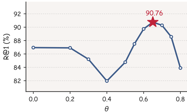
Rerank gate \theta
