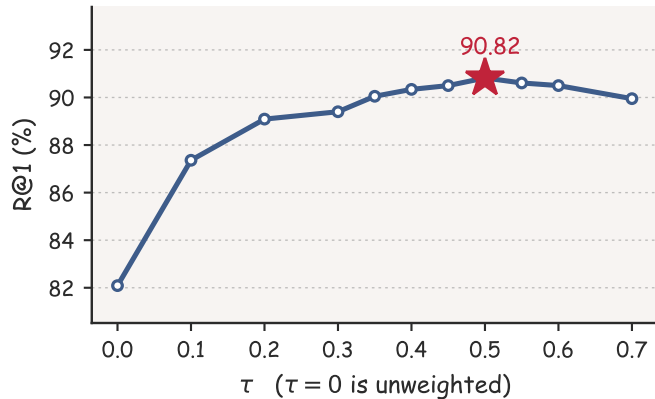
Patch-importance threshold \tau
