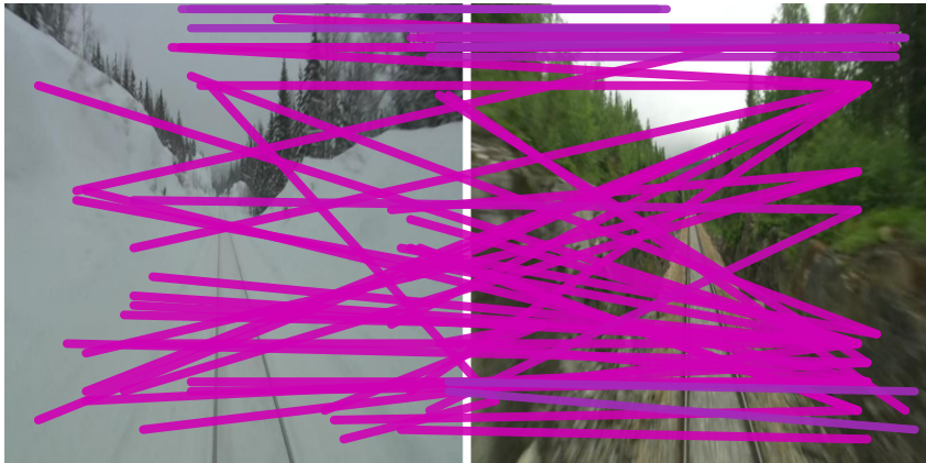
MaxSim, unweighted ( c_i = m_i )
