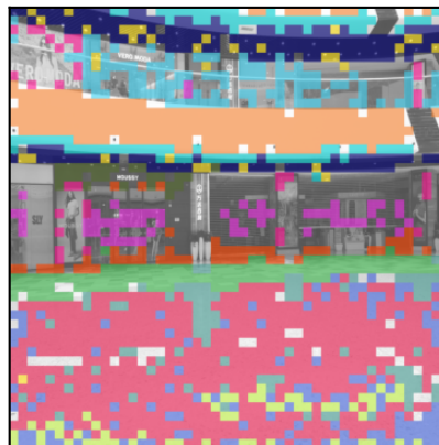
clusters (overlay)
