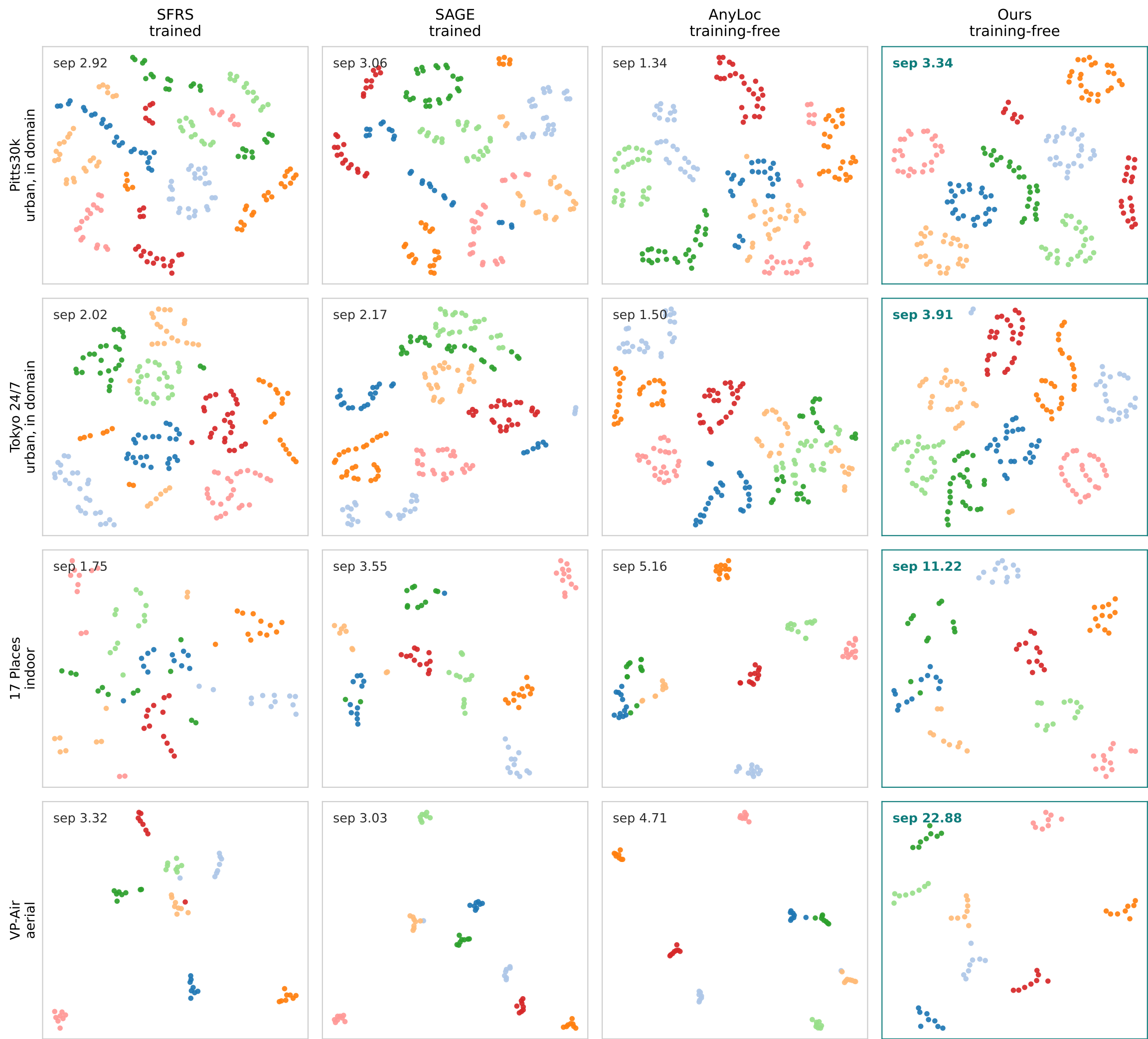
Images of the same place, embedded by each method's own similarity (t-SNE on precomputed distances, perplexity 10, seed 0)
