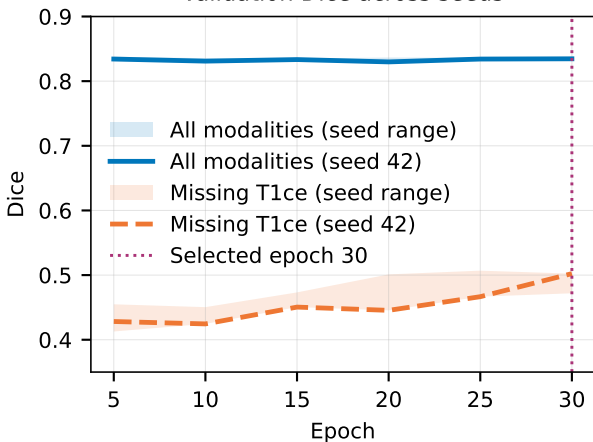
Validation Dice across seeds
