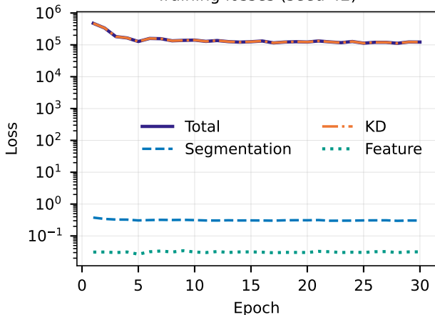
Training losses (seed 42)
