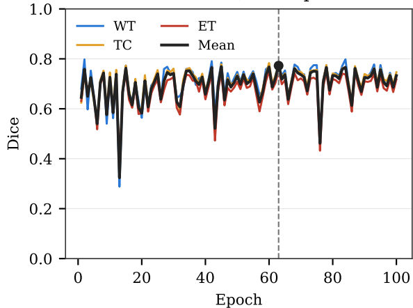
Validation Dice, best epoch 63
