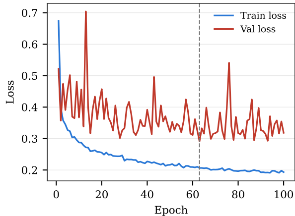
MACAF v2 loss
