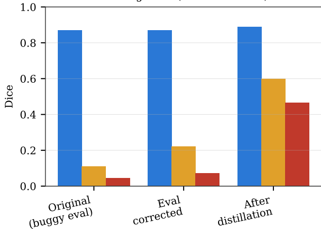
Missing T1ce (T1+T2+FLAIR)
