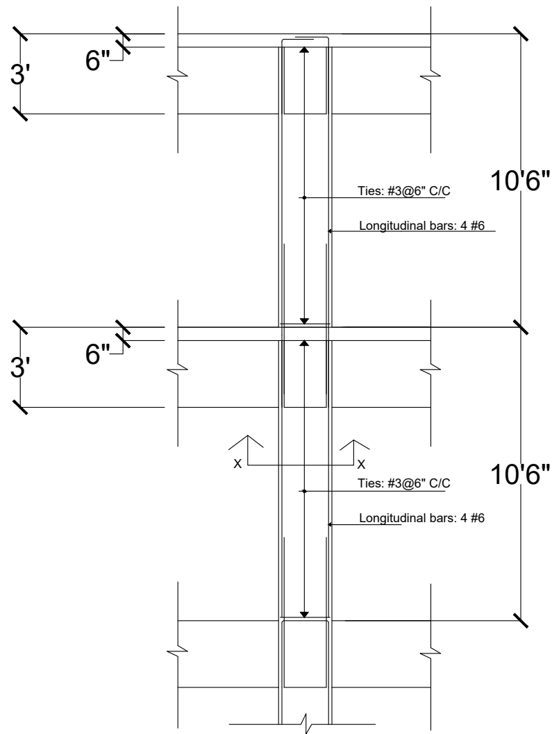
COLUMN ELEVATION (sc 3"=15')
