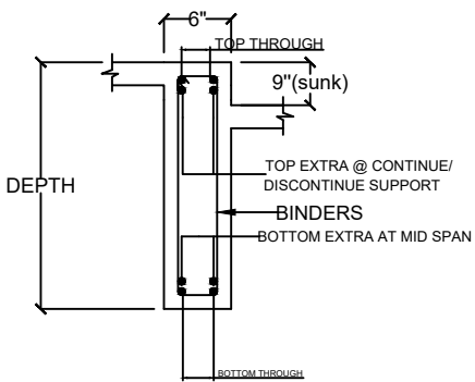
TYP. INTERNAL CONTINUOUS BEAM SECTION FB-02 (6"x30") NTS
