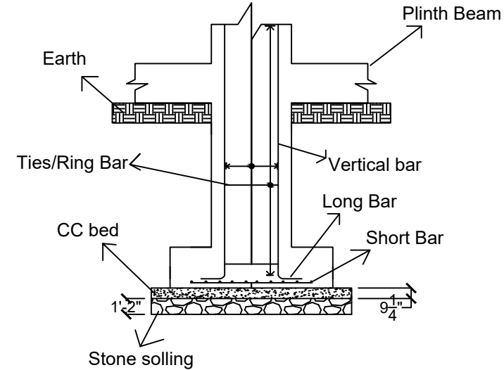
TYPICAL FOOTING DETAILS
