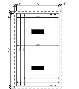
TYP. COMBINED FOOTING
