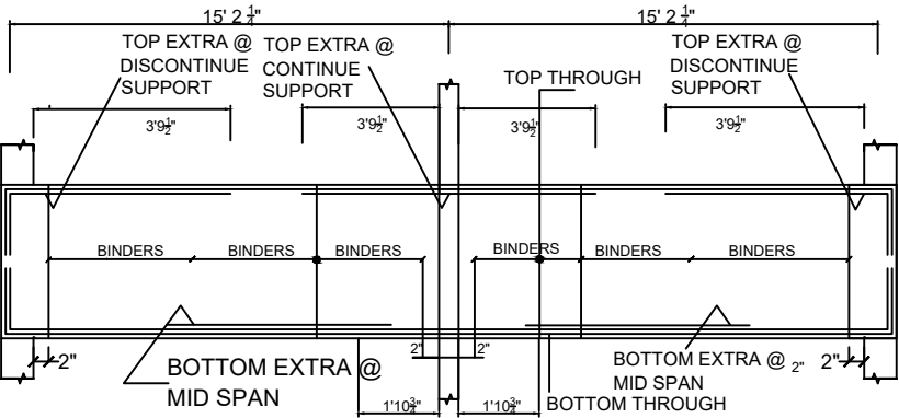
CONTINUOUS BEAM ELEVATION FB-02
