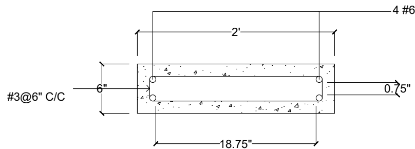
Longitudinal bars: 4 #6 Ties: #3@6" C/C Section X-X of Column (sc 1'=1")
