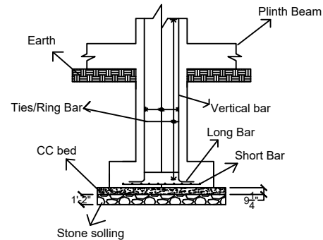
TYPICAL FOOTING DETAILS
