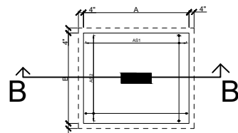
TYP. ISOLATED FOOTING
