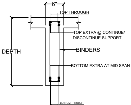
TYP. INTERNAL SIMPLY SUPPORTED BEAM SECTION FB-02 (6"x30") NTS
