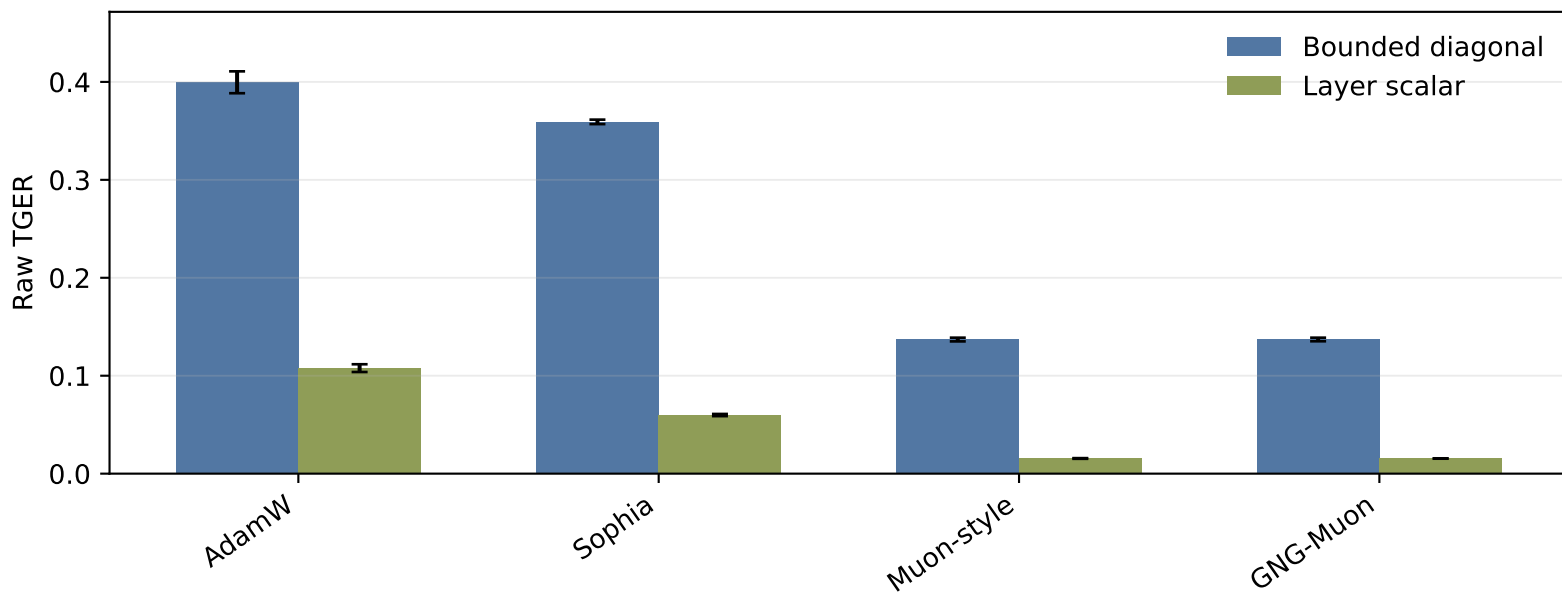
Fashion-MNIST
