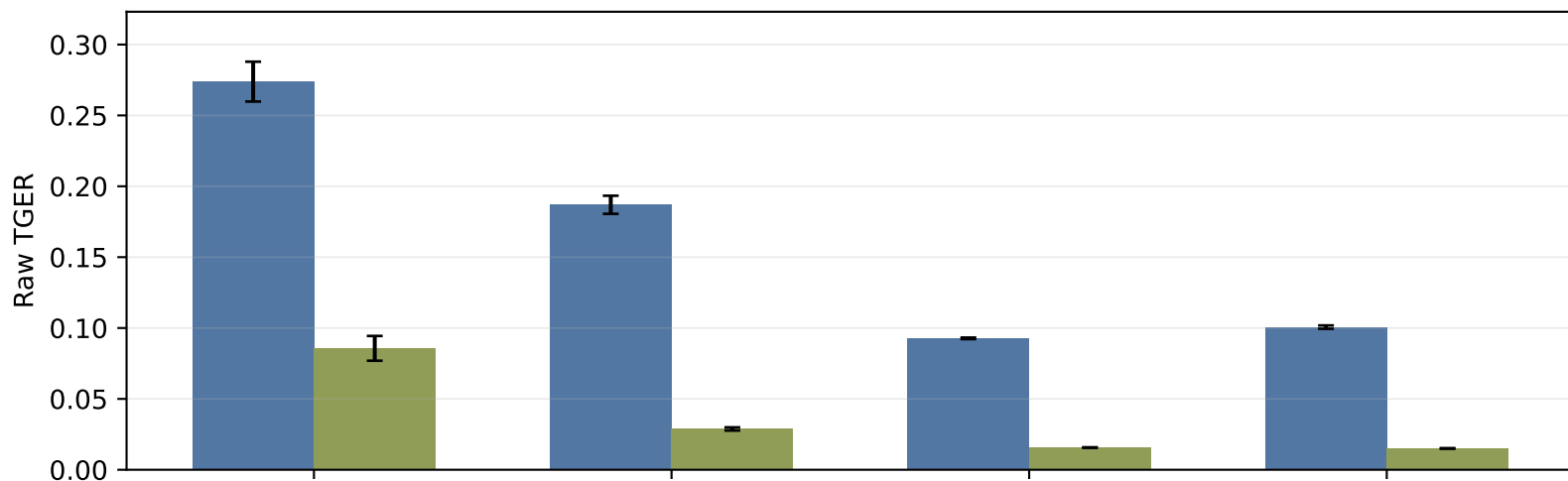
Fashion-MNIST
