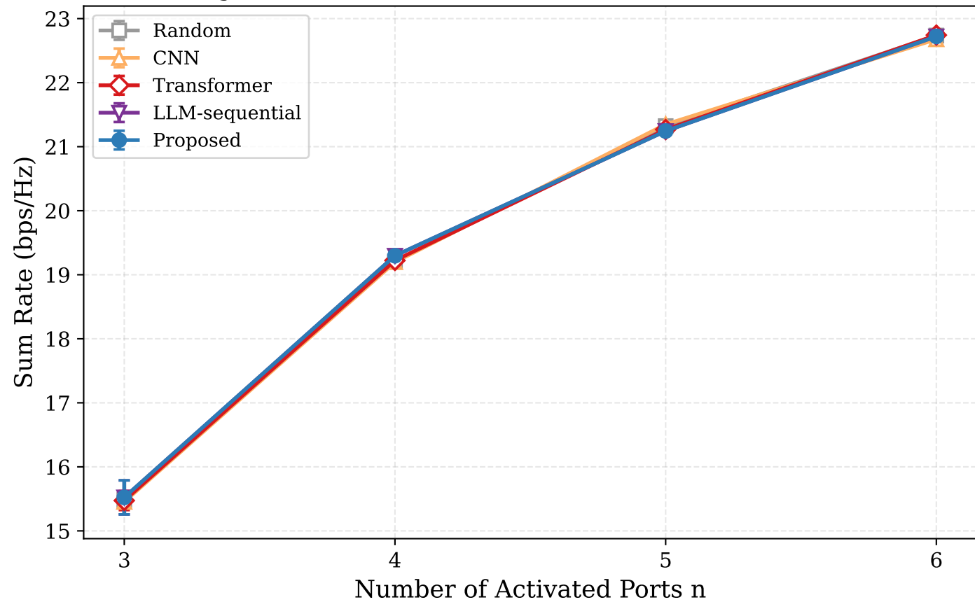
Fig. 8: Sum Rate versus Number of Activated Ports
