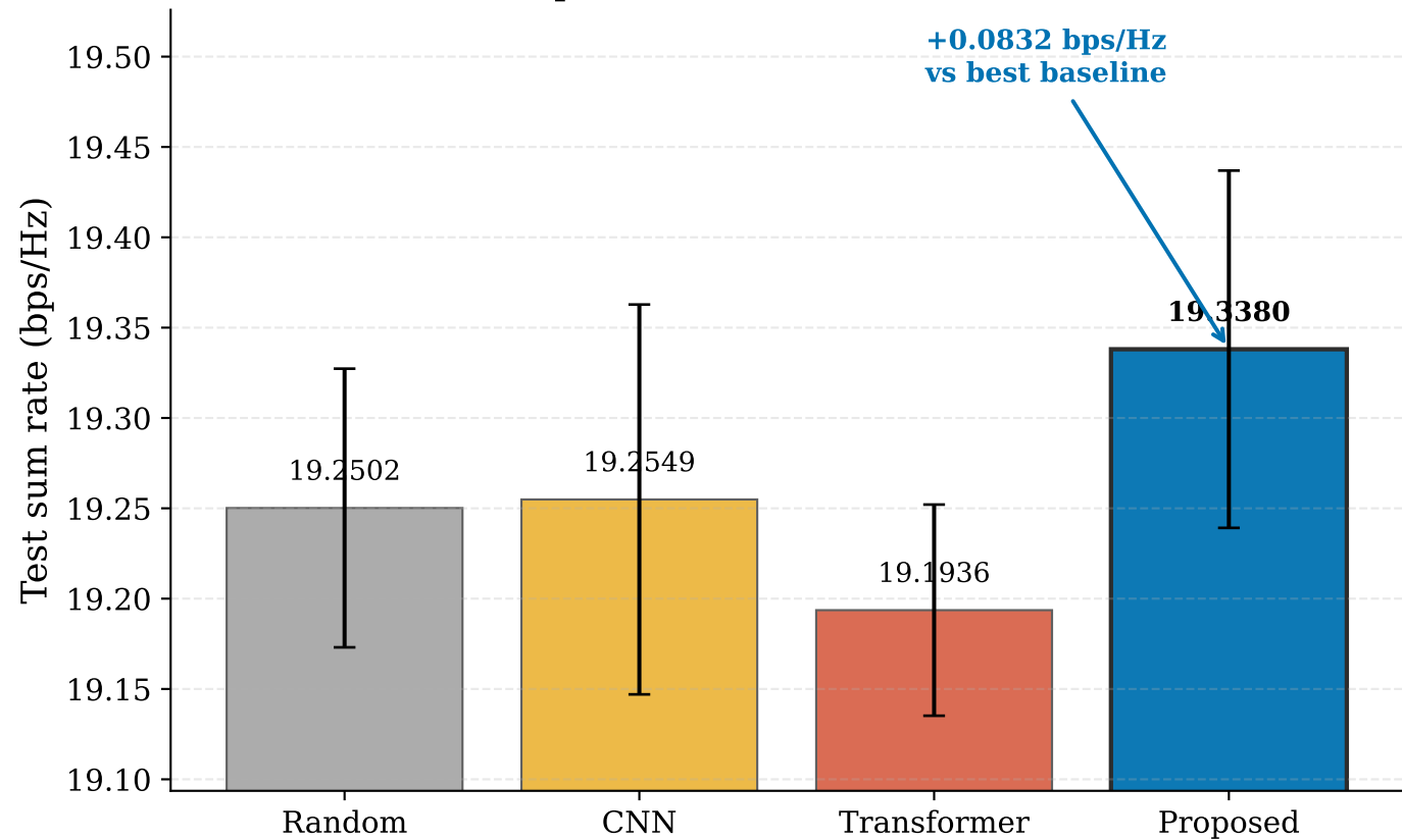
Mean performance across five seeds
