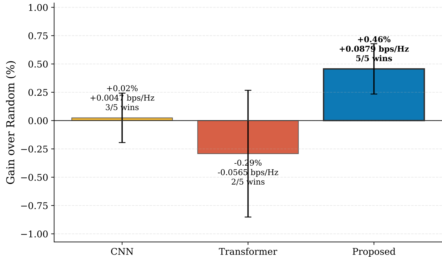
Gain over Random across five seeds
