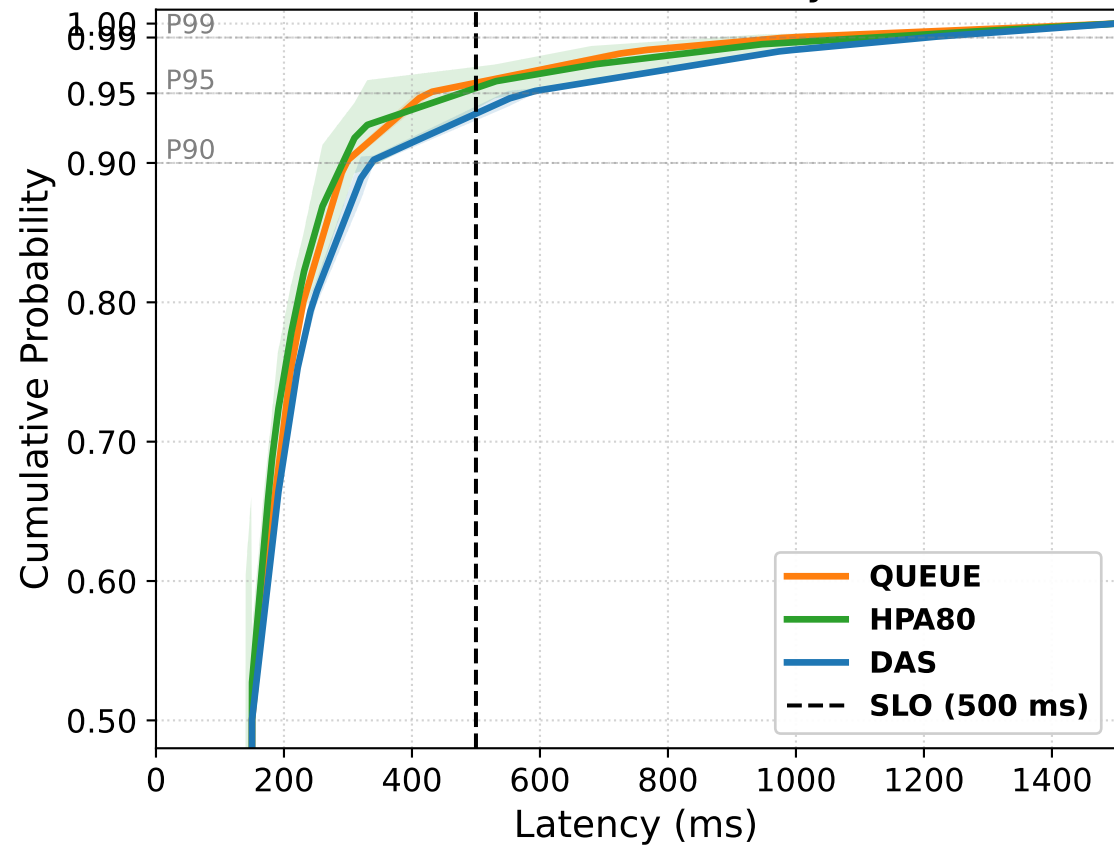
(a) End-to-End Latency CDF
