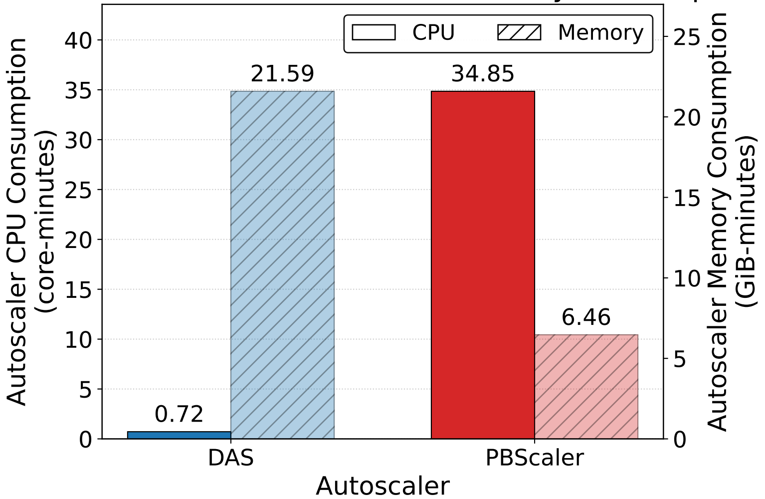
Cumulative Autoscaler CPU and Memory Consumption
