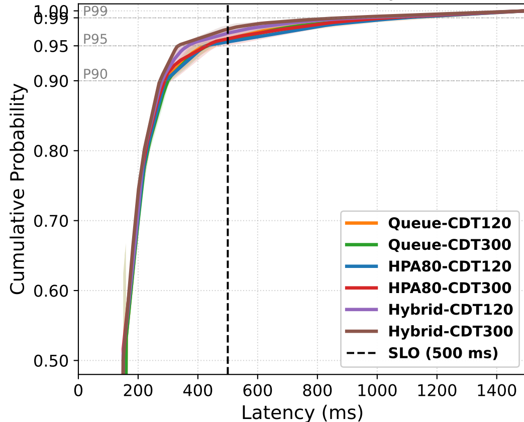
(a) End-to-End Latency CDF
