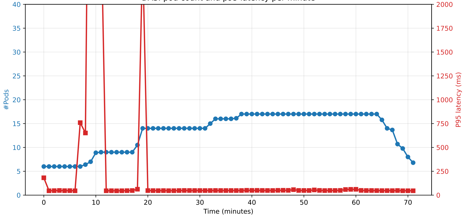
DAS: pod count and p95 latency per minute
