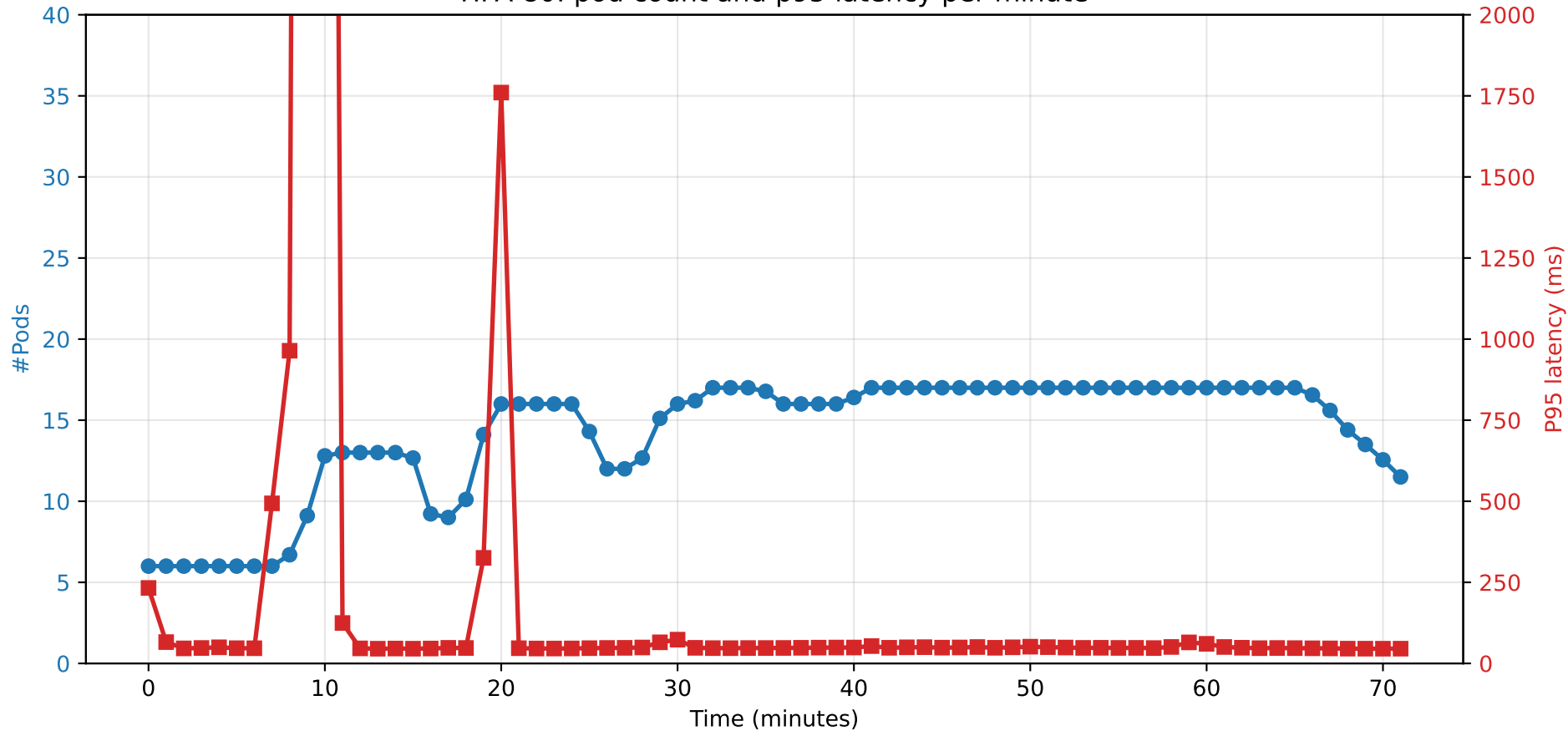
HPA-80: pod count and p95 latency per minute
