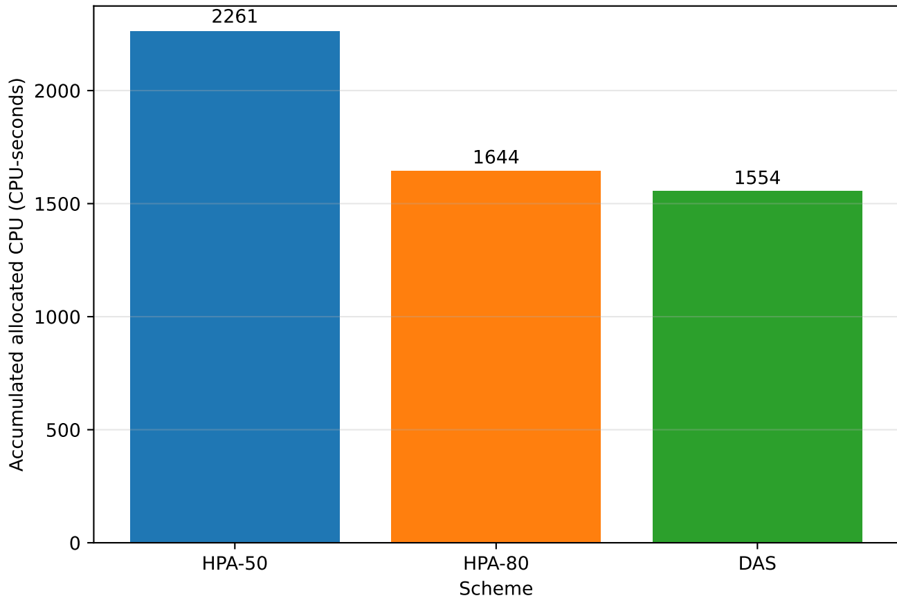
Accumulated allocated CPU of all deployments
