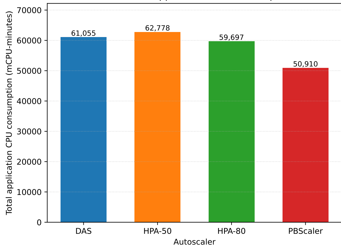
Cumulative Application CPU Consumption
