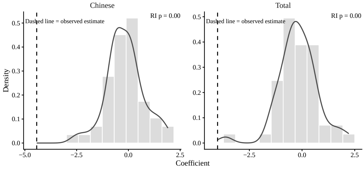
Figure 4: Placebo classroom-reassignment test for peer exposure.
