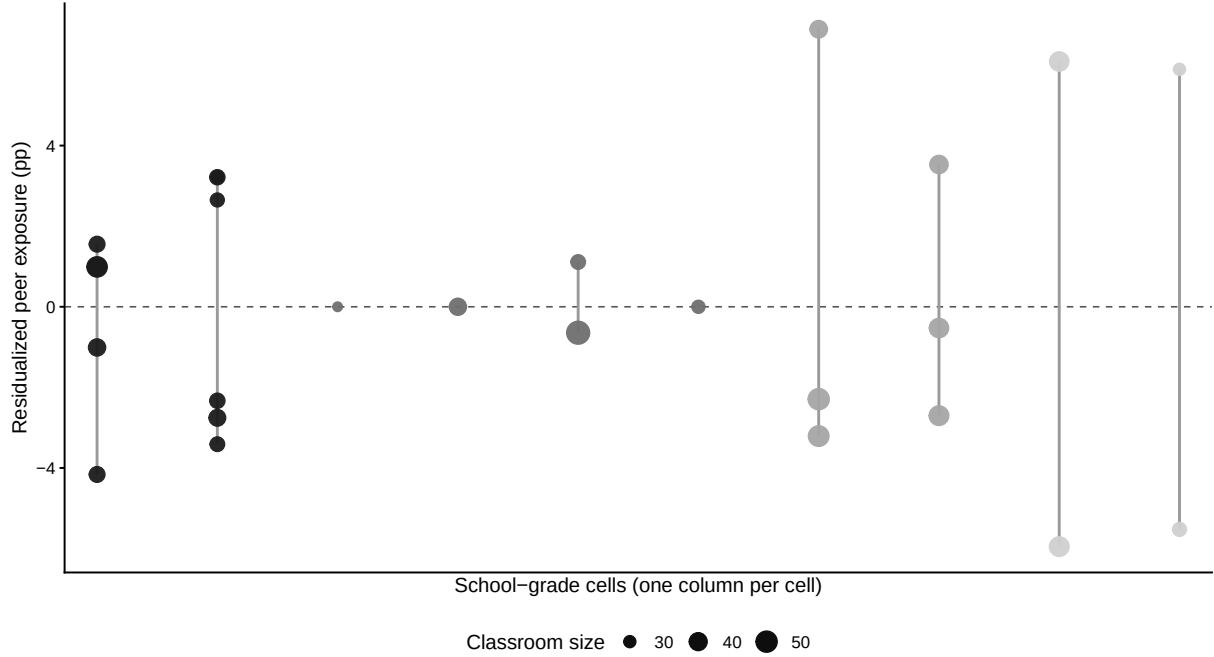
Figure D.2: Residualized variation in classroom peer exposure.
