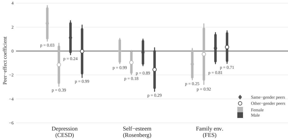
Figure D.8: Same- and other-gender peer effects on psychosocial outcomes, by recipient gender.
