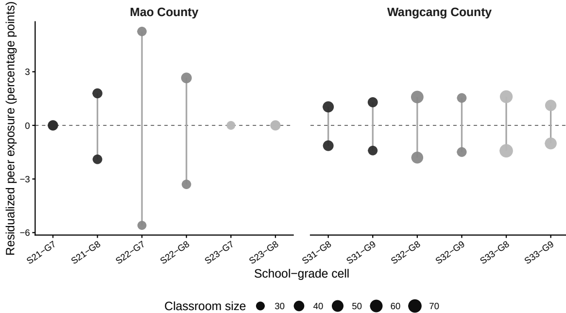
Figure B.2: Residualized variation in classroom peer exposure in Mao and Wangcang.
