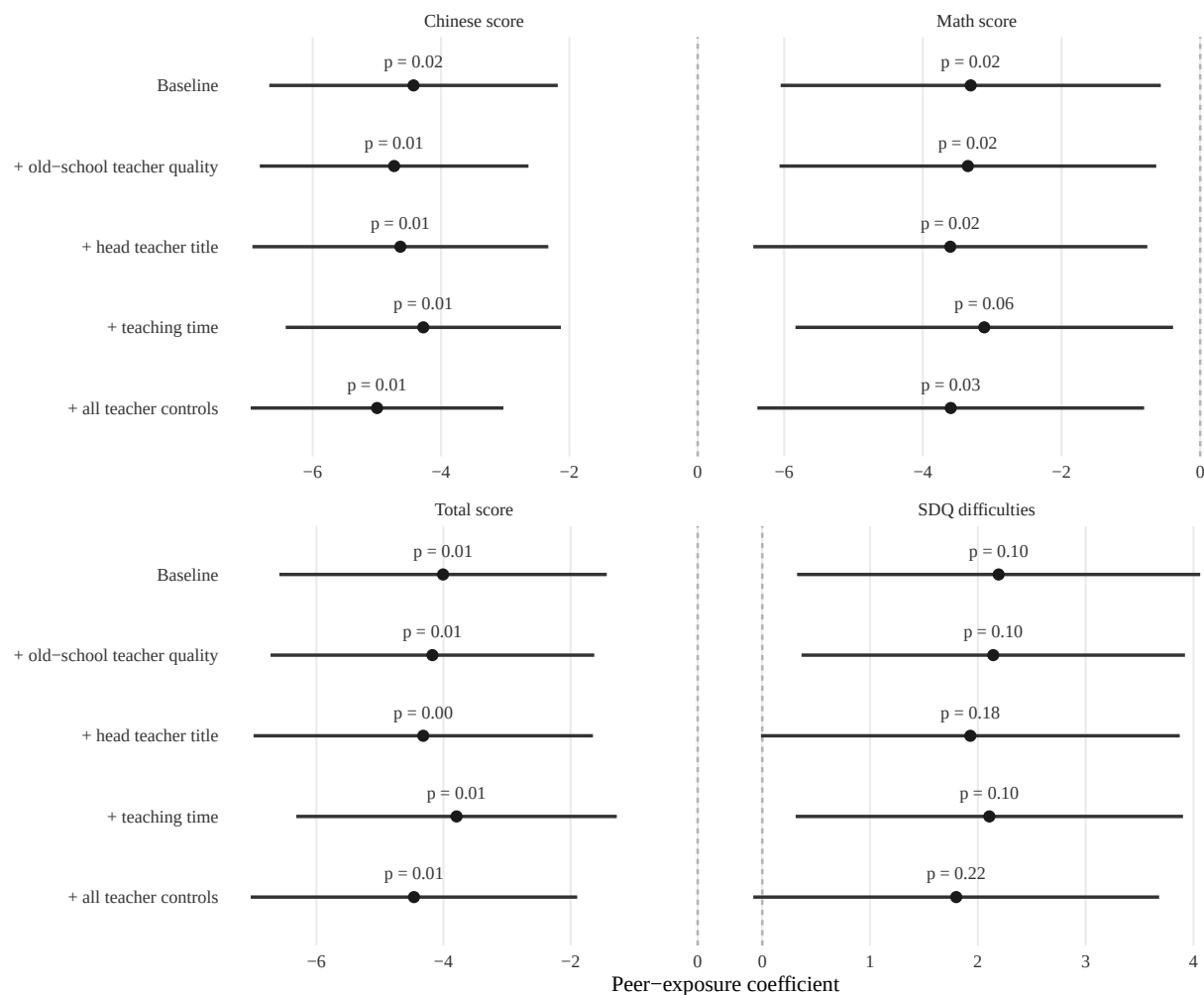
Figure D.10: Peer-exposure estimates with alternative teacher-side controls.
