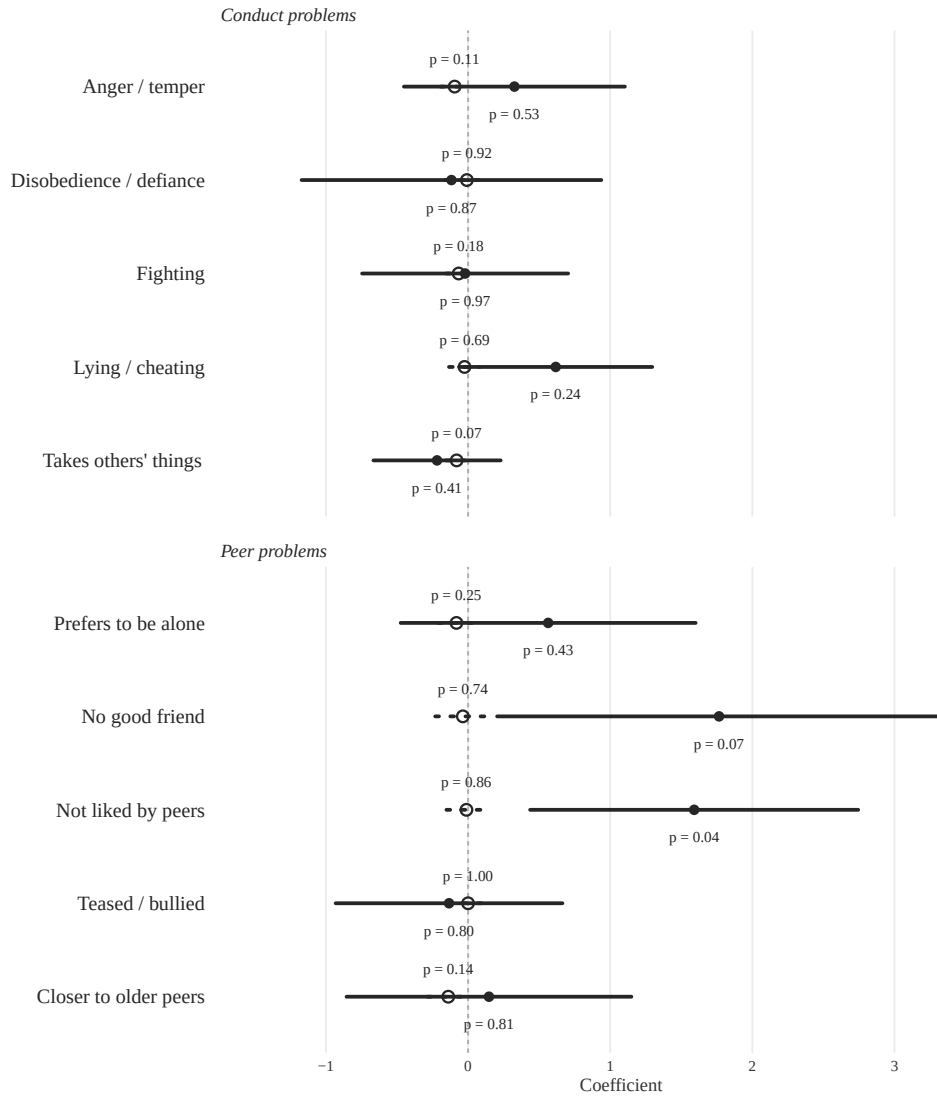
Figure D.7: Item-level SDQ outcomes, by subscale.
