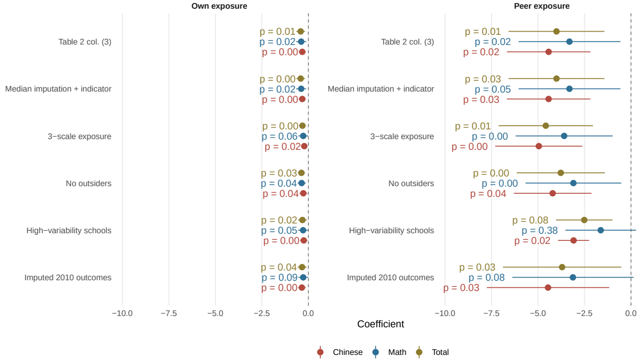
Figure D.4: Sensitivity of peer-exposure estimates to alternative definitions and sample coverage.
