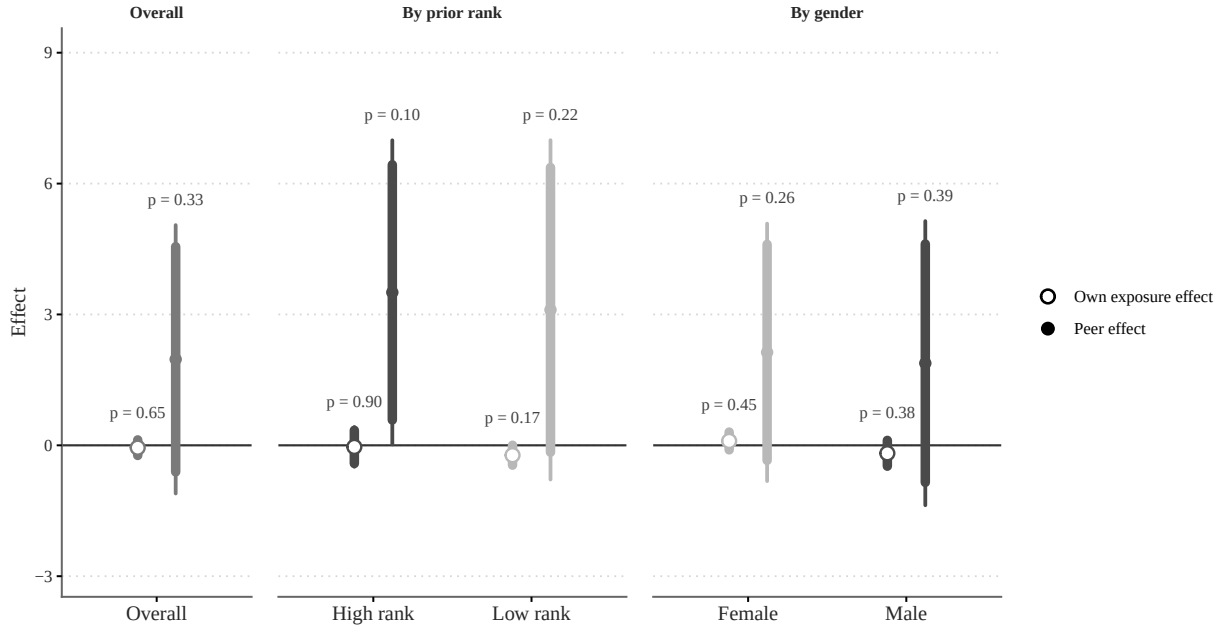
Figure D.9: Study-effort estimates: overall, by prior rank, and by gender.
