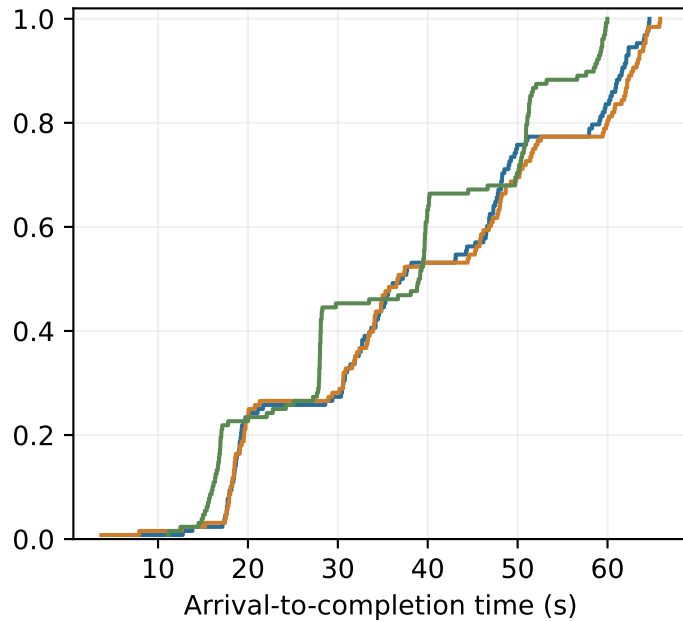
Frozen new inputs: 128 complete requests per arm
