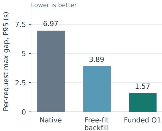
(a) Maximum-gap tail
