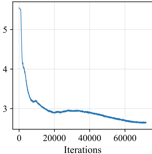
iBOT loss
