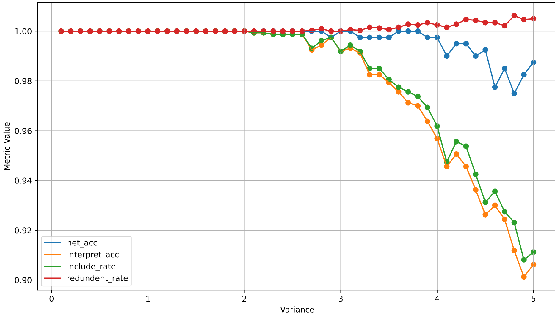
Variance & Metrics
