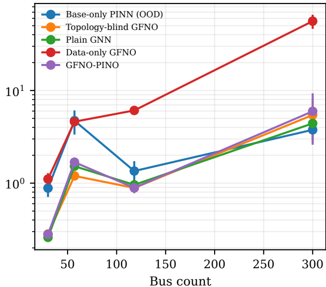
Mean max. power-balance mismatch (p.u.)
