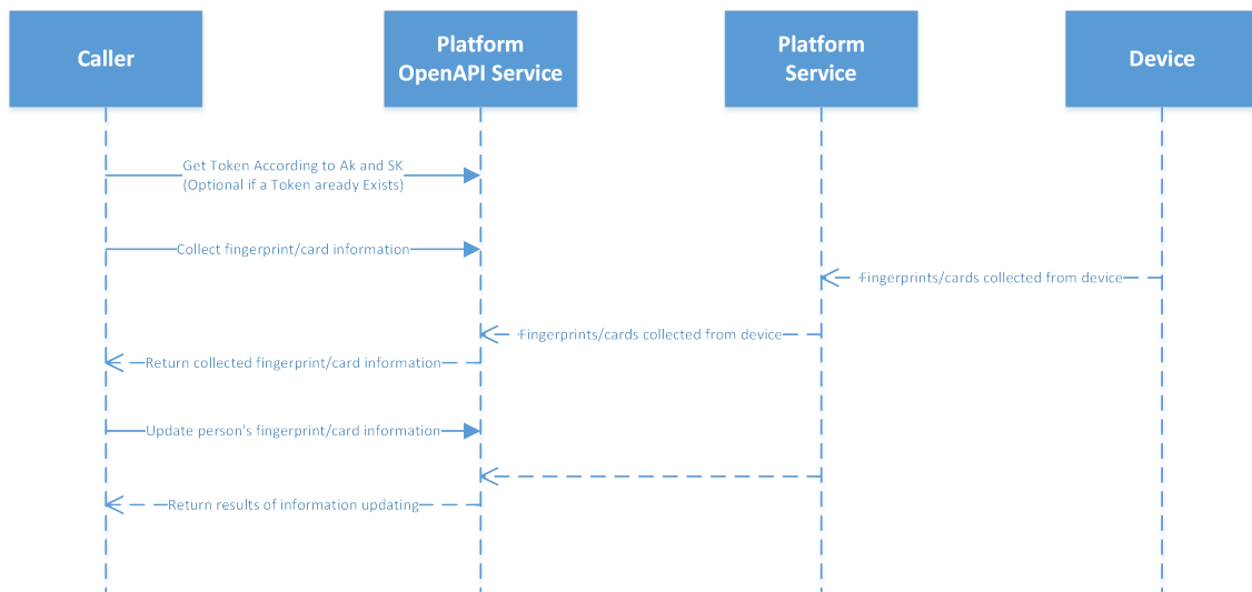
Figure 4-12 Sequence Diagram of Updating Fingerprint/Card Information
