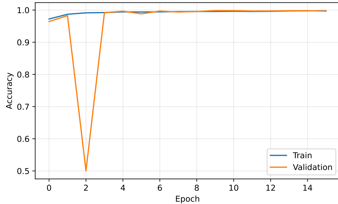
Custom CNN - Accuracy
