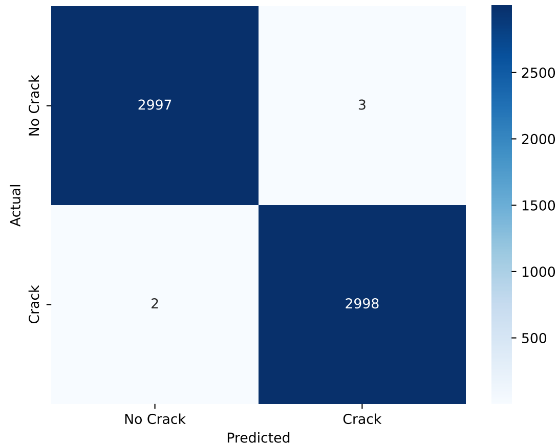
MobileNetV2 - Confusion Matrix
