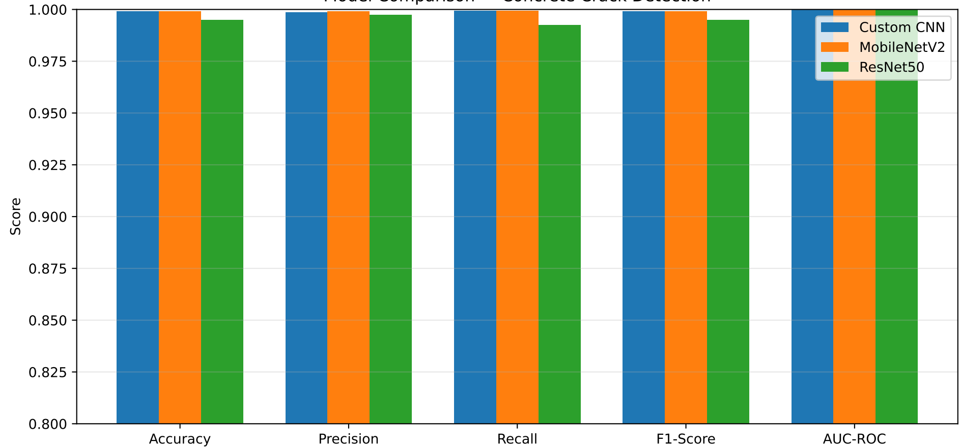
Model Comparison — Concrete Crack Detection
