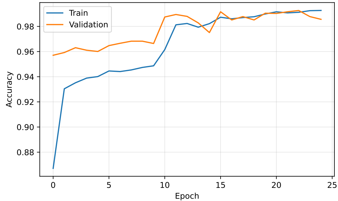
ResNet50 - Accuracy
