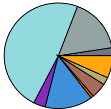
t\bar{t} + \geq 2b CR 1
