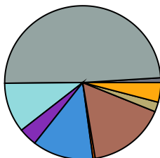
t\bar{t} + \geq 1c CR
