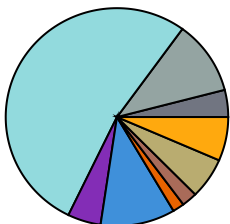
t\bar{t} + \geq 2b CR 3
