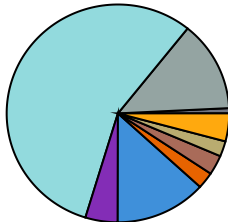
STXS 2 SR
