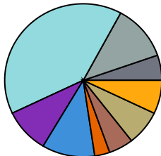
STXS 6 SR
