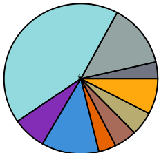
STXS 5 SR
