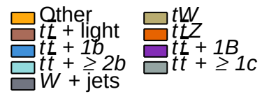
STXS 4 SR
