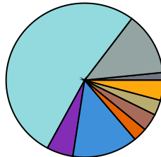
STXS 3 SR
