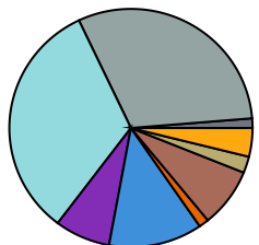
Boosted CR
