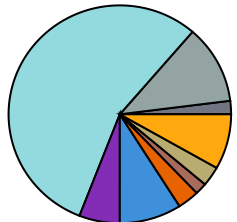
Boosted SR
