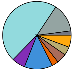
STXS 4 SR
