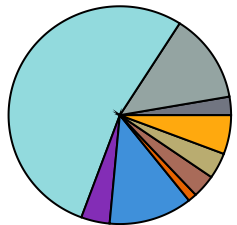
t\bar{t} + \geq 2b CR 2
