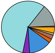
STXS 1 SR
