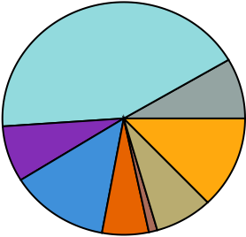
STXS 5 SR
