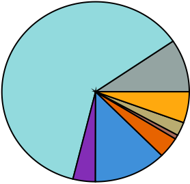
STXS 2 SR
