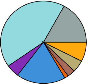
t\bar{t} + \geq 2b CR
