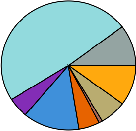
STXS 4 SR
