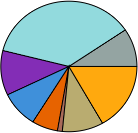
STXS 6 SR
