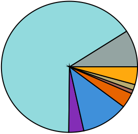
STXS 1 SR
