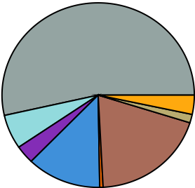
t\bar{t} + \geq 1c CR
