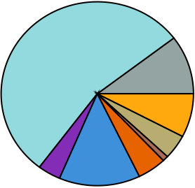
STXS 3 SR
