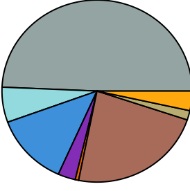
t\bar{t} + \geq 1c region
