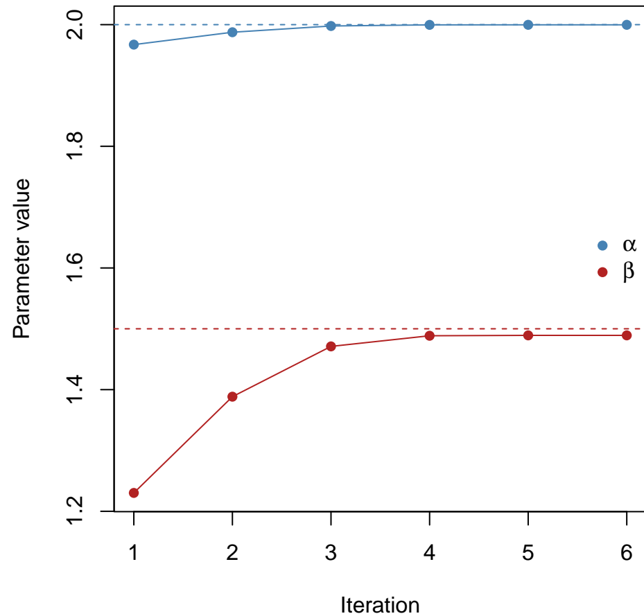
Newton-Raphson convergence
