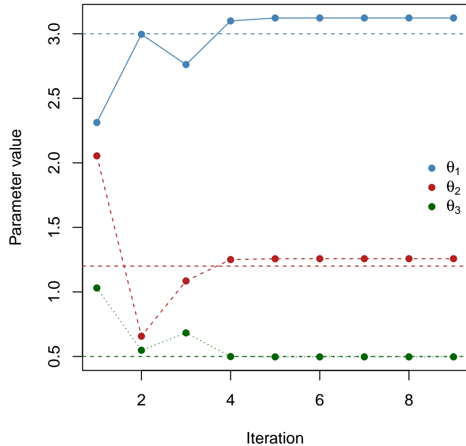
Gauss-Newton convergence
