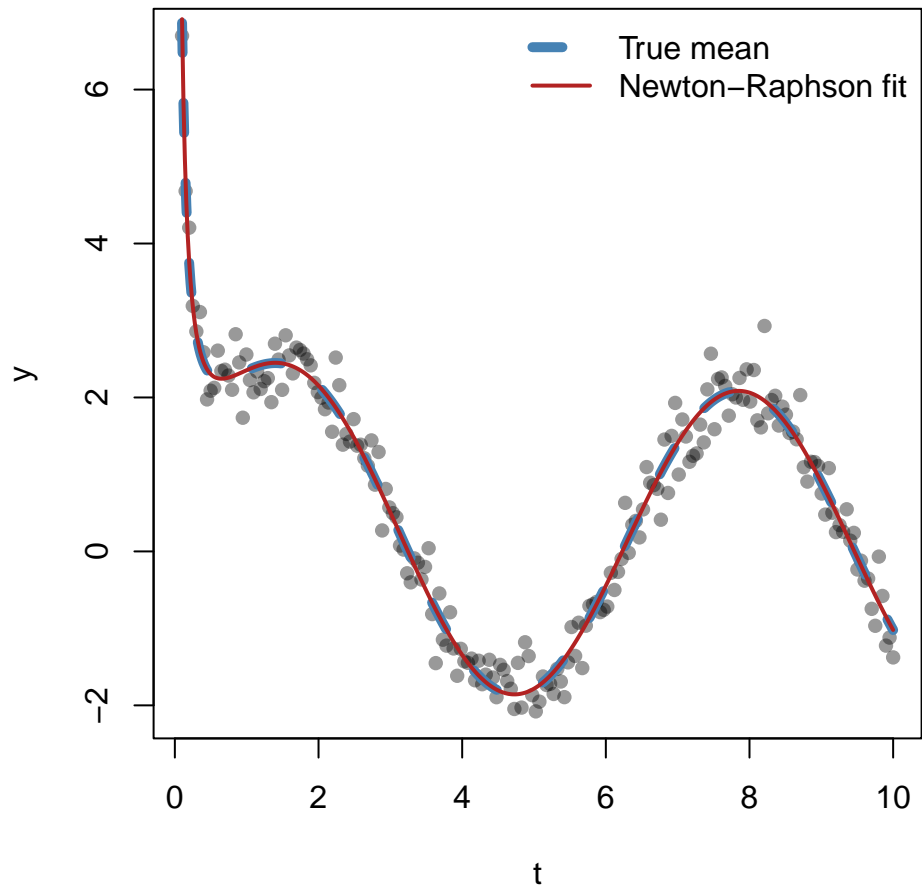
Non-linear fit via Newton-Raphson
