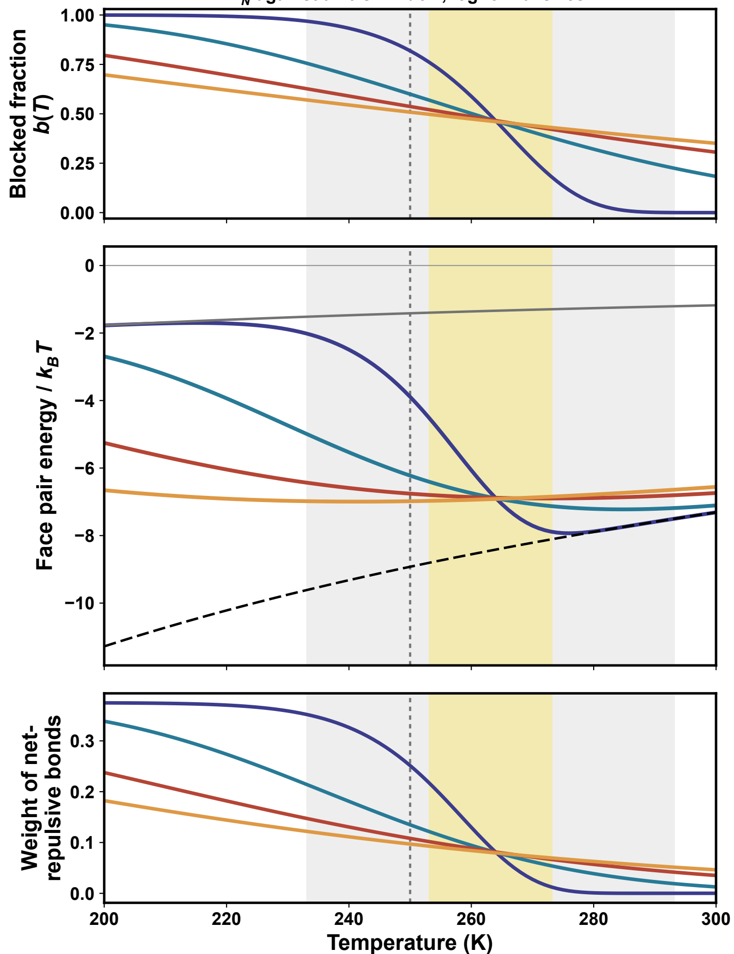
Gradual dipole freeze-in on cooling, fixed face contact \tau_N against a 20 s window, lognormal sizes
