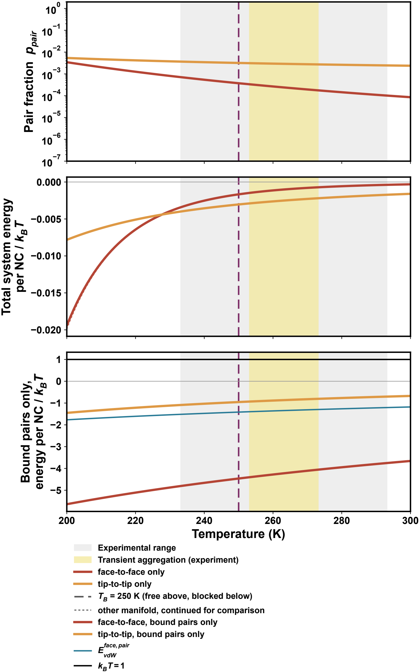
Restricted single-channel assembly, dimer face twist tolerance \delta = 1^\circ (costs face 8.19\,k_B T against tip), \phi = 0.01
