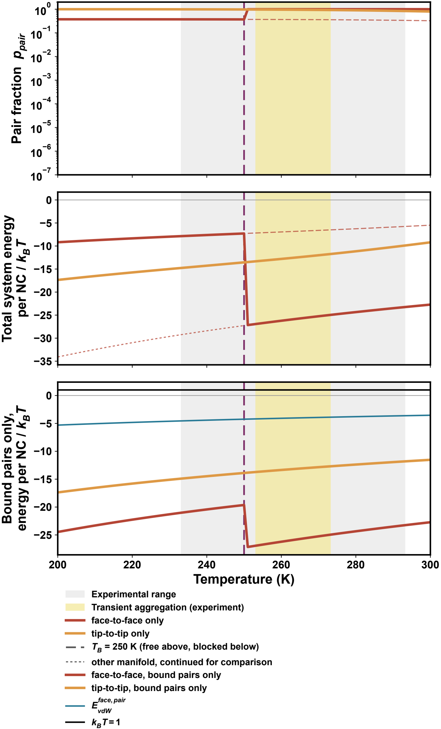
Restricted single-channel assembly, superlattice face twist tolerance \delta = 5^\circ (costs face 4.97\,k_B T against tip), \phi = 0.01
