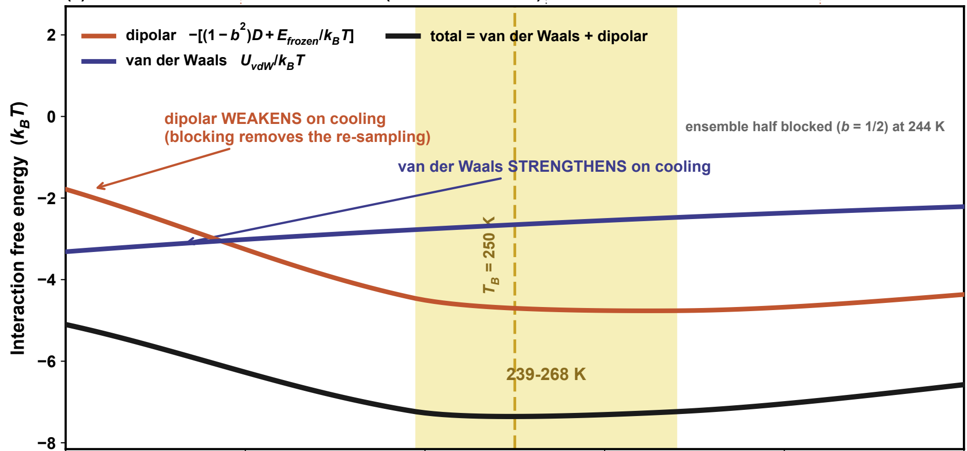
(a) The two attractions and their sum (coordination z = 1 )
