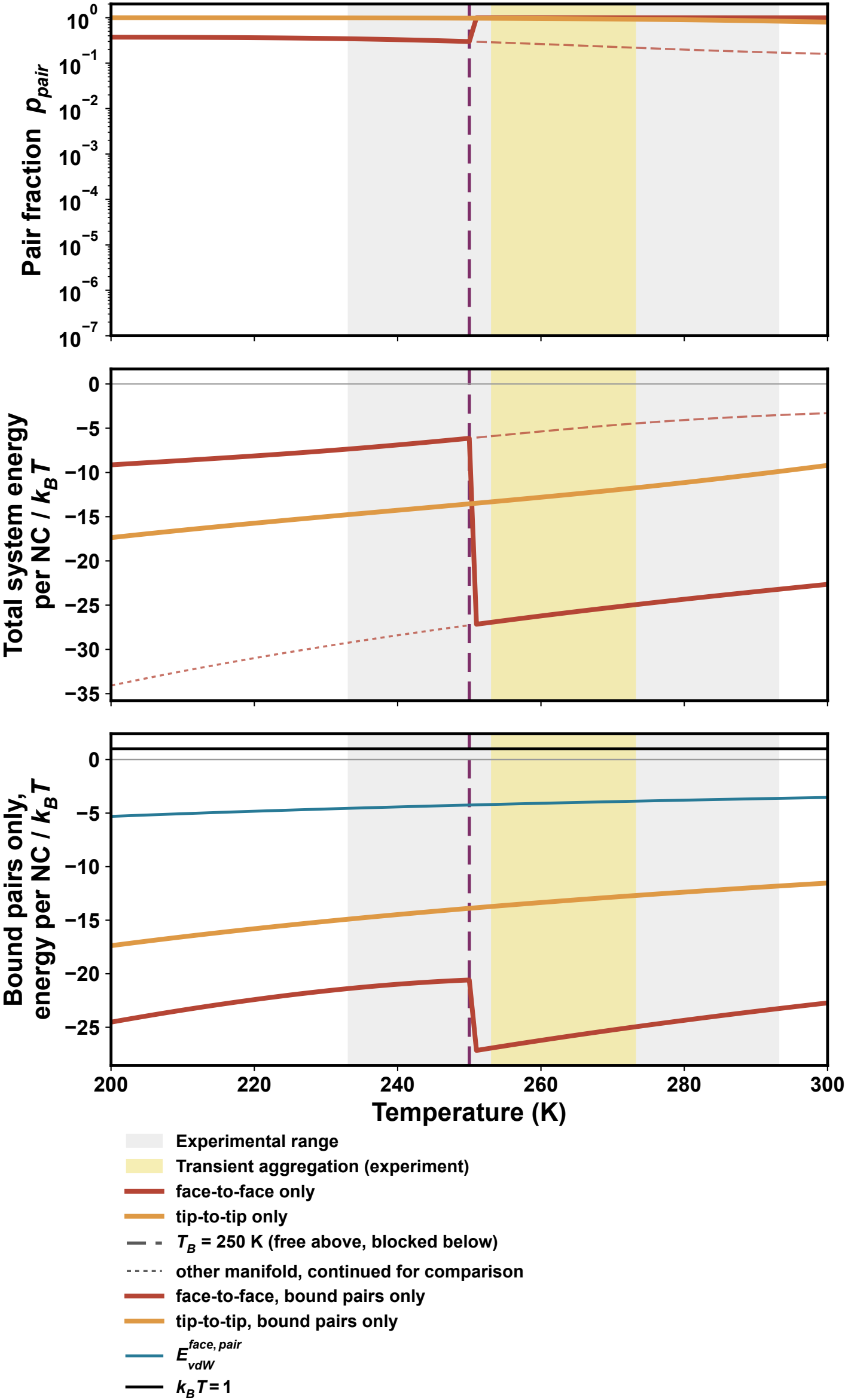
Restricted single-channel assembly, superlattice face twist tolerance \delta = 1^\circ (costs face 8.19\,k_B T against tip), \phi = 0.01
