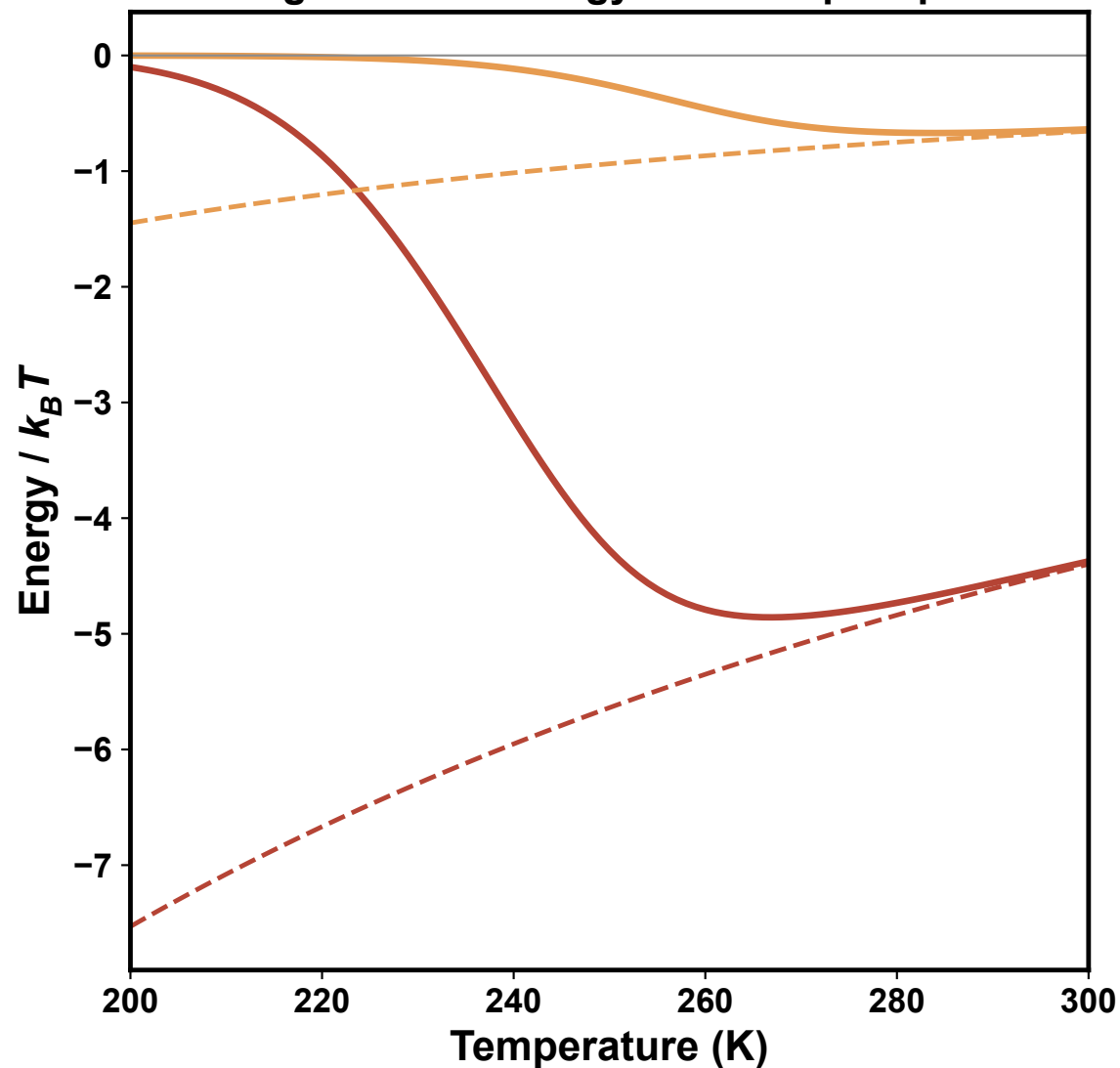
Magnetic free energy vs uncoupled pair
